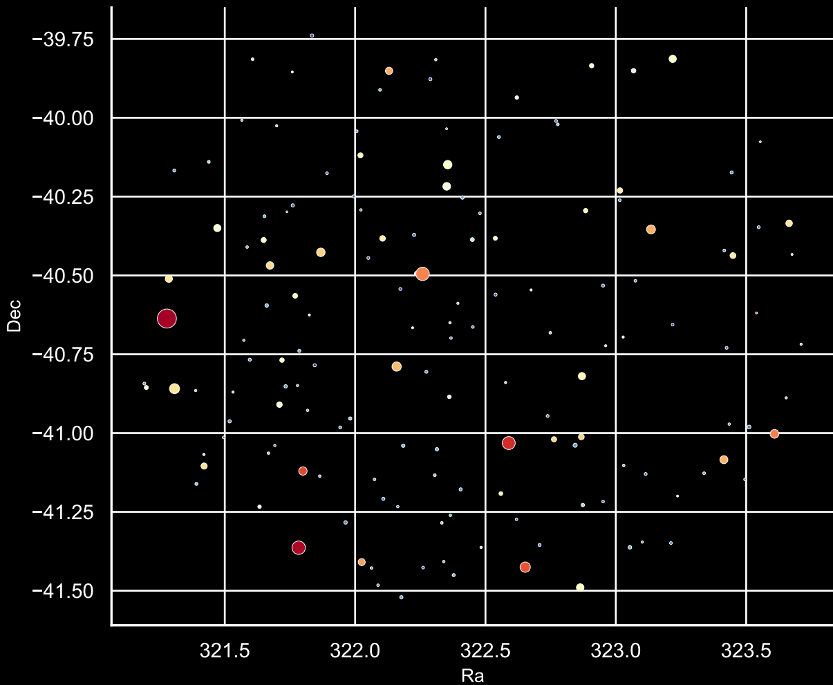
Field [18] Ra [322.36] Dec [-40.7] Stars: 151
