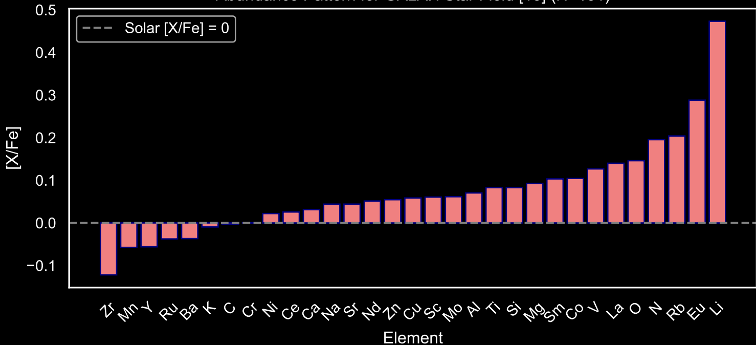
Abundance Pattern for GALAH Star Field [18] (N=151)
