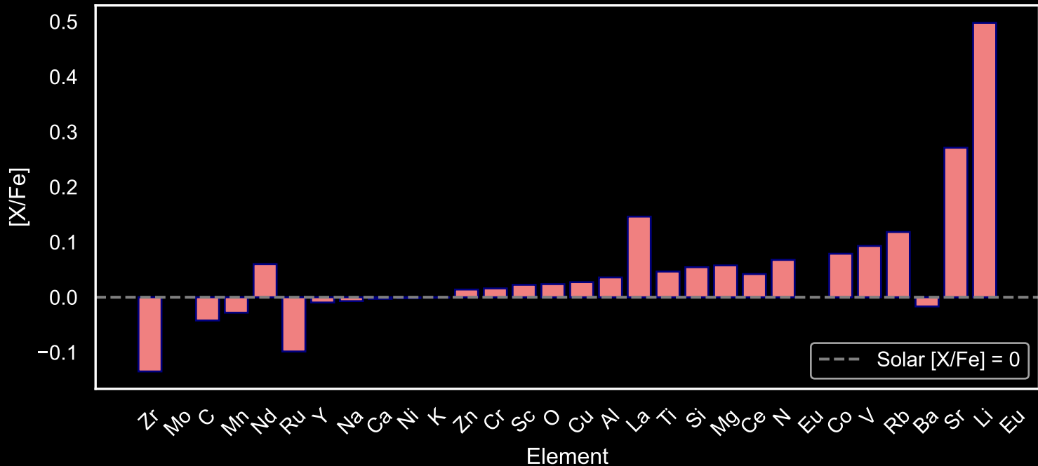
Abundance Pattern for GALAH Main Sequence Stars: Star Field [18] (N=65)
