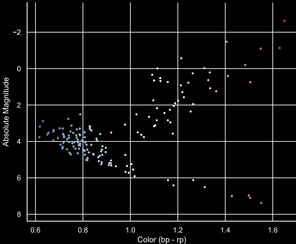
GALAH Hertzprung-Russel Diagram Field [18] Ra [322.36] Dec [-40.7]
