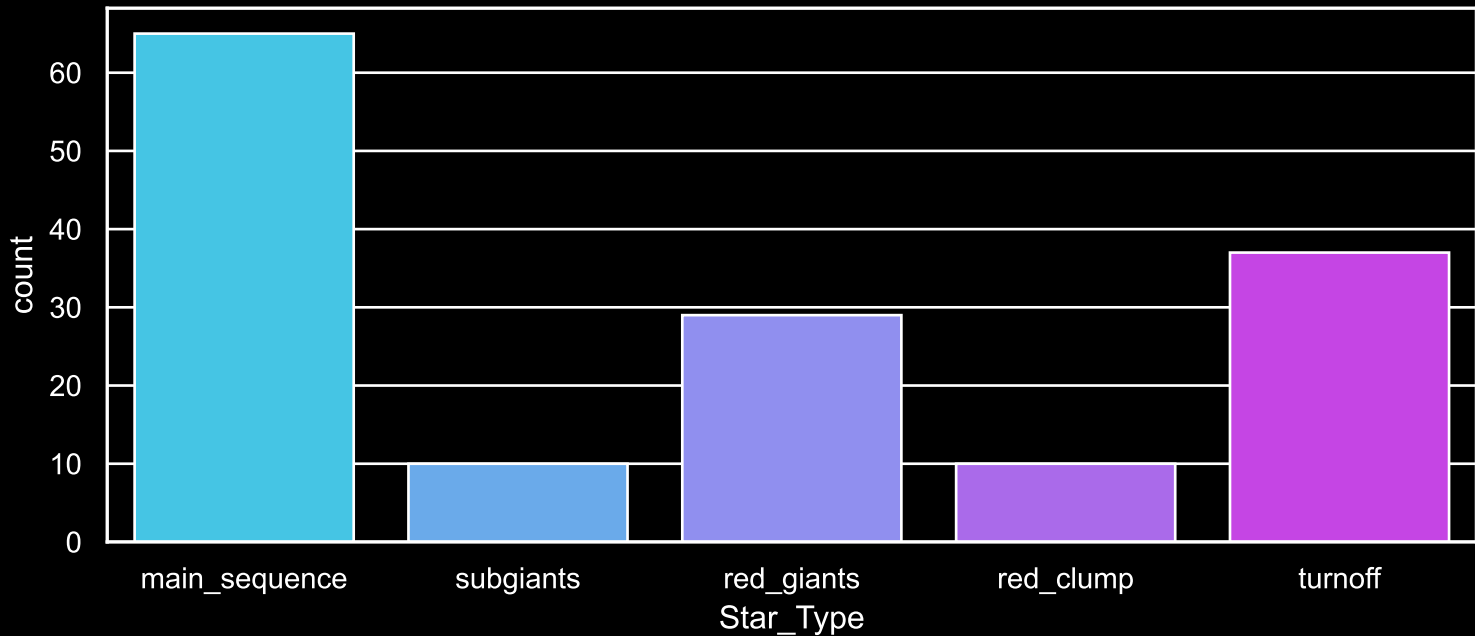
Field [18] Count plot of Star Type
