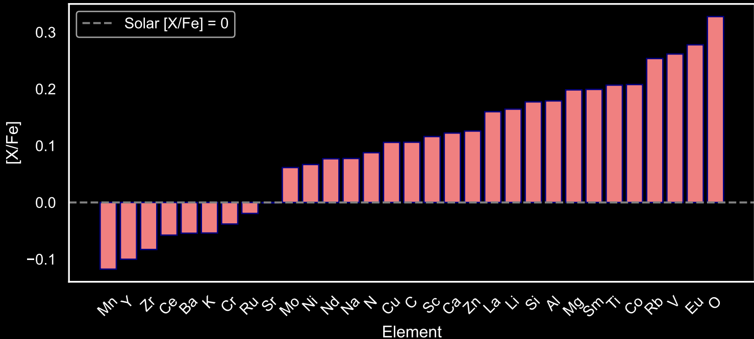
Abundance Pattern for GALAH Red Giants: Star Field [18] (N=39)
